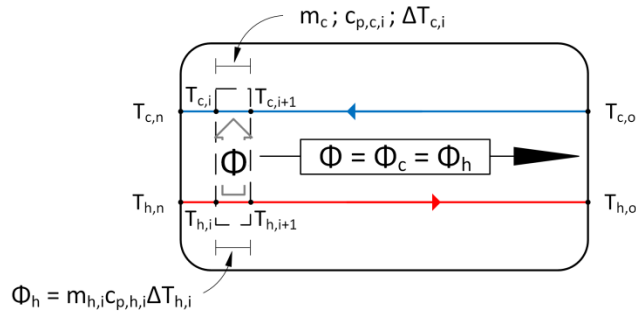
216 217 Figure 4. Schematic of modelling approach for the cold box.
